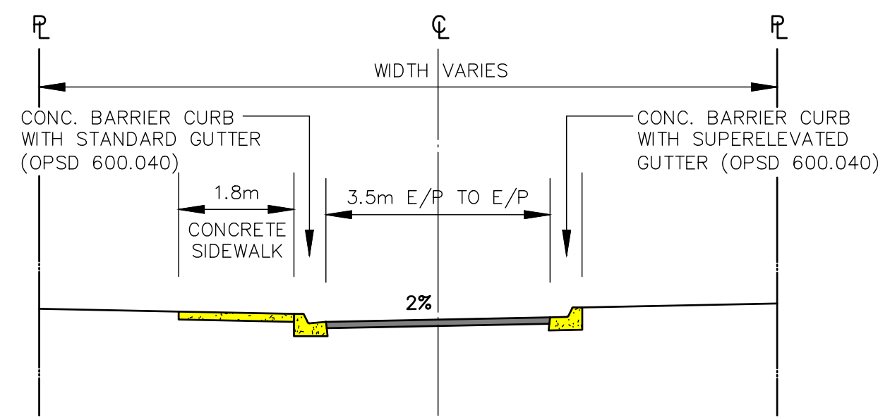
ROAD SECTION – VICTORIA CRESCENT HENDERSON STREET TO SMITH STREET N.T.S.
